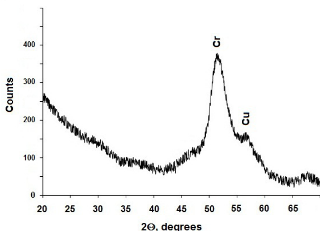
Fig. 8. Typical X-ray spectrum of a coating deposited from the bath containing \text{CrCl}_3 + 2.5\text{ChCl} + 15\text{H}_2\text{O} at 7 \text{ A dm}^{-2} and 40^\circ\text{C} .
